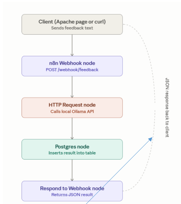
Figure 95: Note the response back to client
