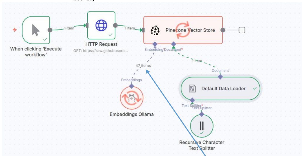
Figure 73: Our workflow to save data to vector store. 47 items possibly mean that 47 chunks were processed till now. Chunk size for Recursive text splitter is 512 as selected embedder is:
