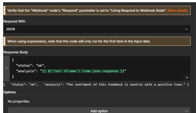
Figure 99: Respond to webhook node
