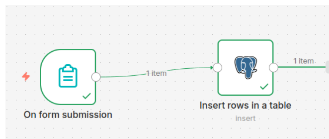
Figure 42: Form entering data into postgres
