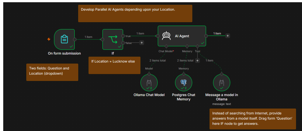
Figure 15: This AI Agent DOES NOT have a chat node. Neither also it answers questions from Internet.
