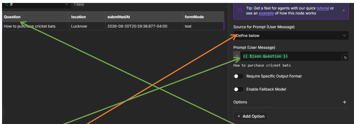
Figure 17: AI Agent configuration (this MUST be selected as 'Define below'). And drag Question from the left panel to Prompt. You can, of course, write appropriate System messages
