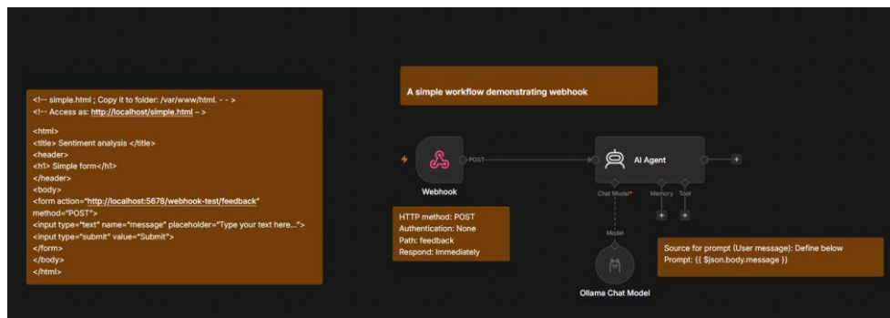
Figure 92: A simple webhook demo. IT is called by an html form on Apache webserver. Ollama chat model: llama3.2
