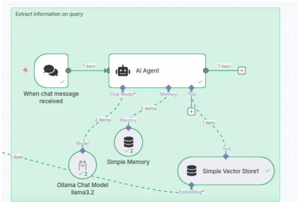
Figure 66: Querying a vector store
