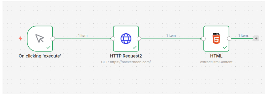
Figure 91: HTTP request and HTML nodes are configured as above.
