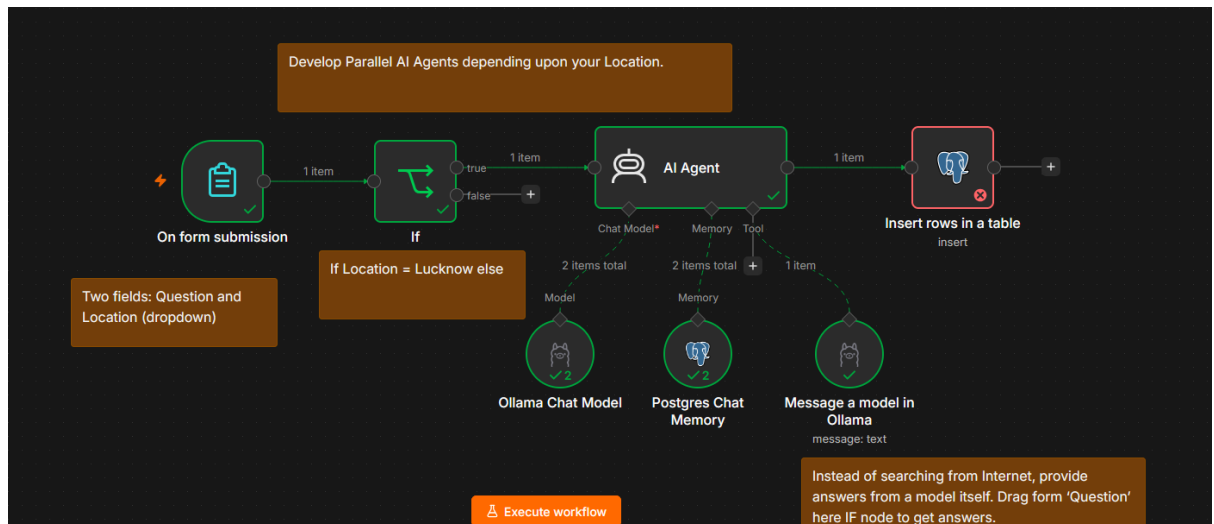
Figure 16: Insert a postgresql table at the end to receive data
