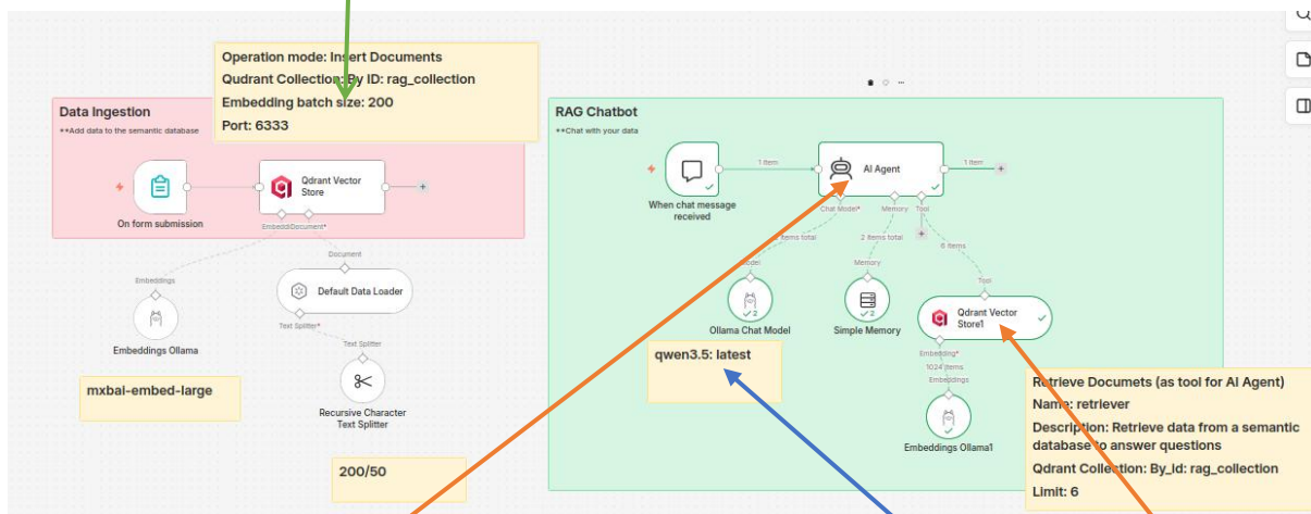
Figure 68: Write a proper System Message. The Collection ID name should be the same in both the branches. Also give a proper name to Retriever tool (such as: 'retriever'). Or, use a small ollama cloud model: minimax-m3:cloud; llama3.2 also works.
