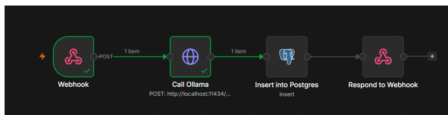
Figure 93: The flow. Call Ollama is HTTP Request node
