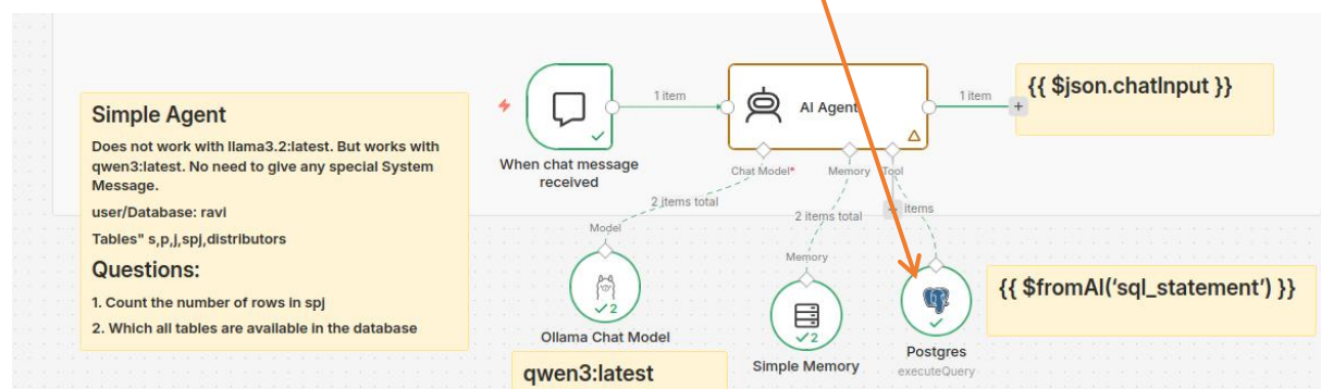
Figure 44: User is ravi, password is ravi and database is ravi. The database contains the standard C J Date's tables: s,p,j,spj and an additional table : distributors. Model: gwen3.5:0.8b also works
