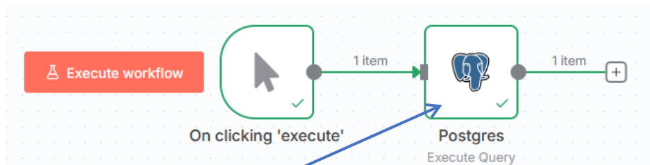
Figure 36: Double click to open it. In Query write: select * from acars ; OR select * from employees ;
