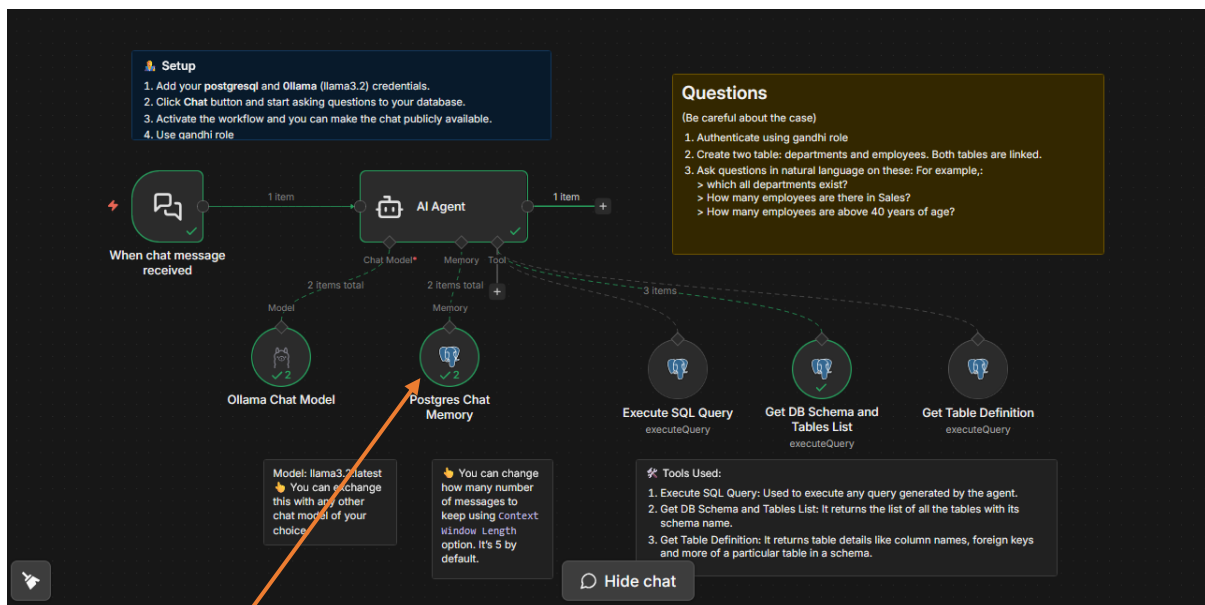
Figure 46: Replace chat history by PG Chat memory. The PostgreSQL account or credentials can be the same as in other PG nodes. In PG Chat memory, you can specify your own table name.
