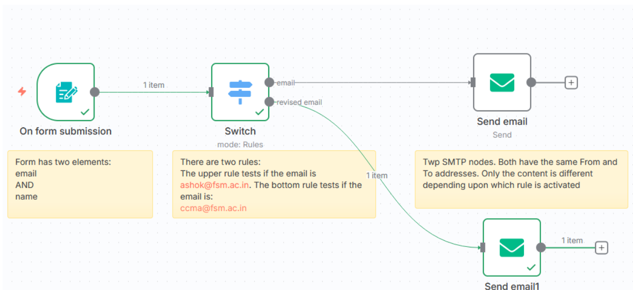
Figure 30: Configuration for switch node is as below.
