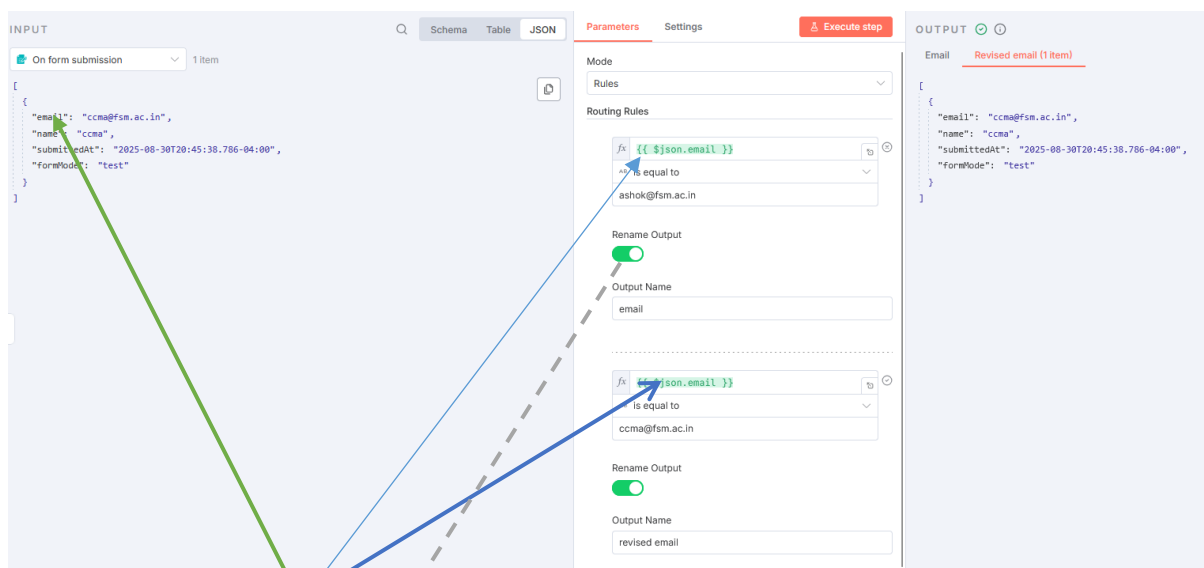
Figure 31: Input element of email is tested in the two rules. Upper rule tests for ashok@fsm.ac.in and the lower rule tests for ccma@fsm.ac.in . In both cases, rename your branches appropriately.
