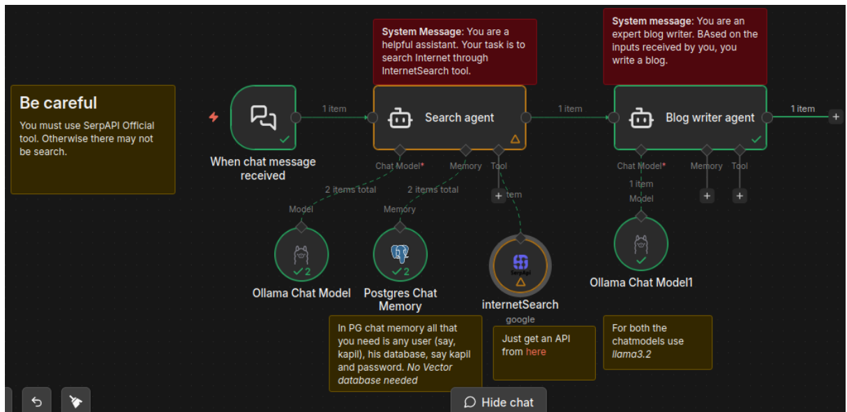
Figure 86: Blog Writer agent needs special configuration. See below.
