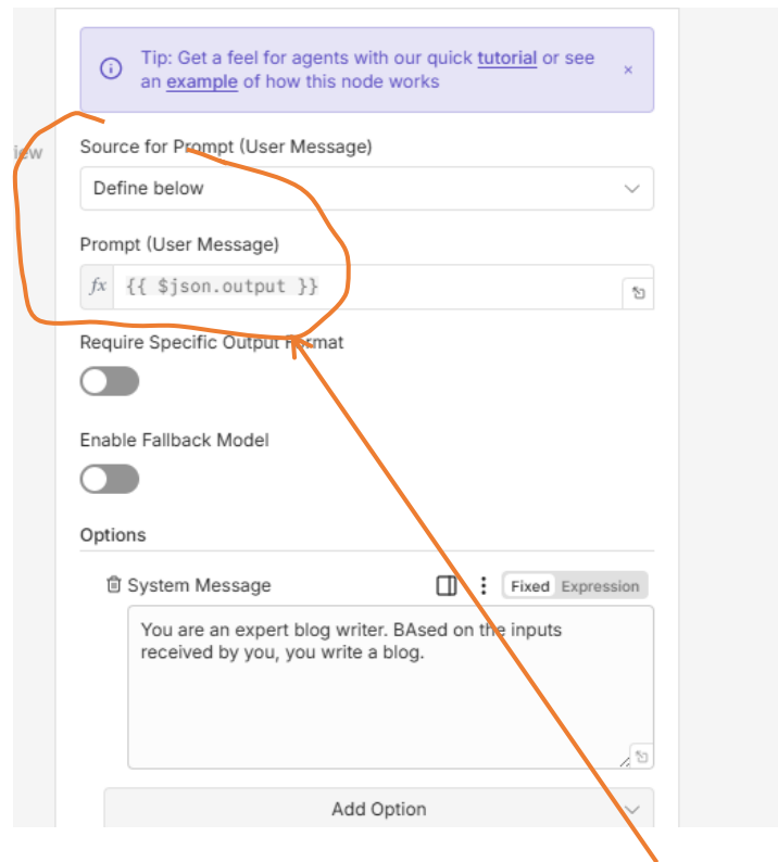
Figure 88: Blog Writer Agent: Besides System Message, make changes here.
