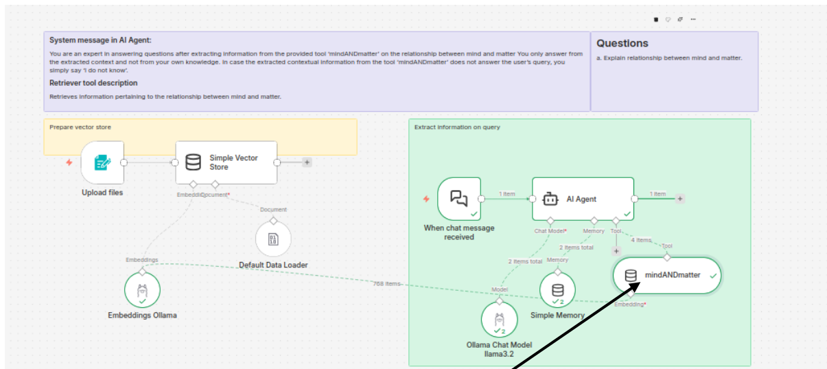
Figure 59: Full workflow. NOTE that even though this is also Simple Vector Store but has been renamed as per the subject.
