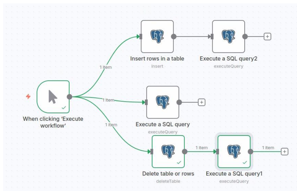
Figure 40; Workflow using different postgres nodes: Execute SQL Query, Insert rows, Delete table of rows
