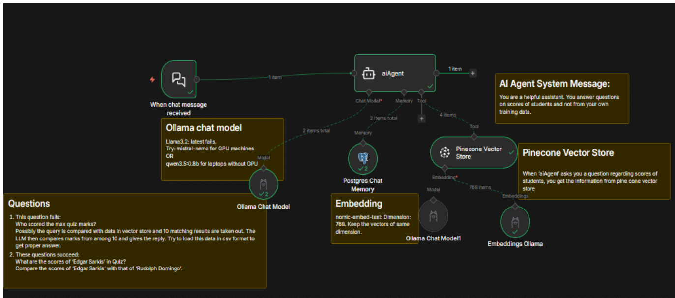
Figure 74: Reading vector data from Pinecone vector store
