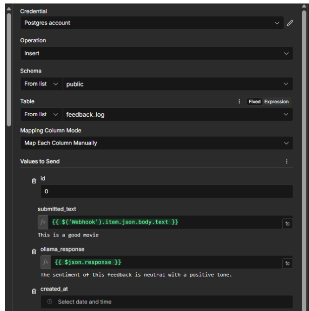
Figure 98: Postgres node
