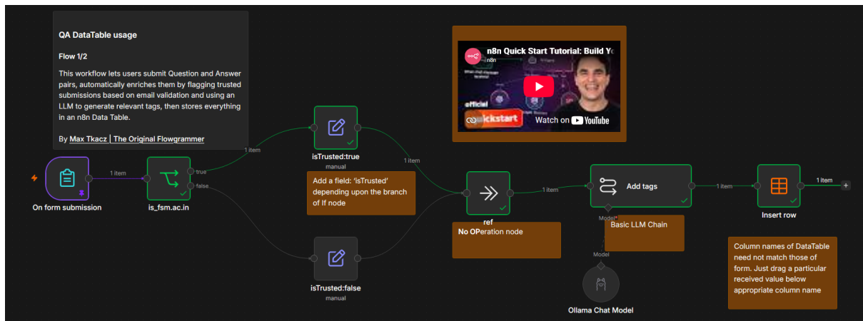
Figure 100: isTrusted node on true branch of if, appends a column isTrusted with value true. On the false branch value added is false.
